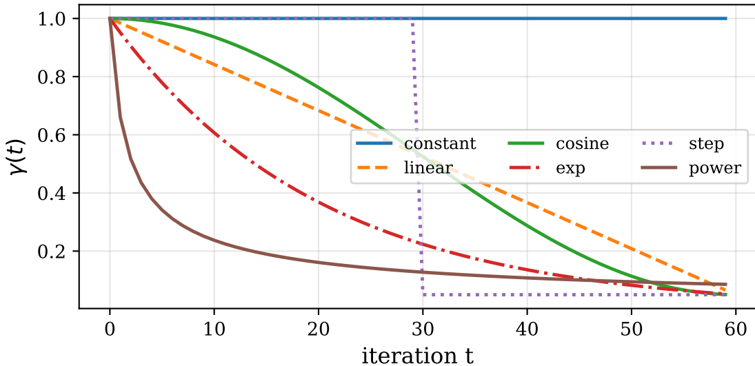
\gamma(t) schedules ( \gamma_{\text{init}}=1.0 , \gamma_{\text{final}}=0.05 , \beta=0.6 )
